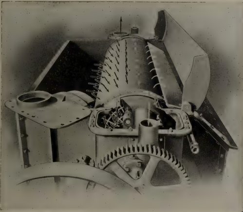
Pneumatic Action of the Save-All
